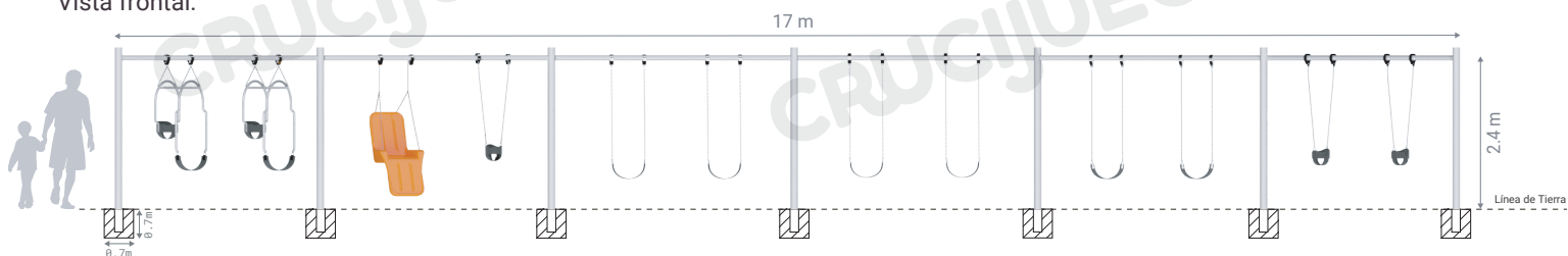
Vista frontal:
